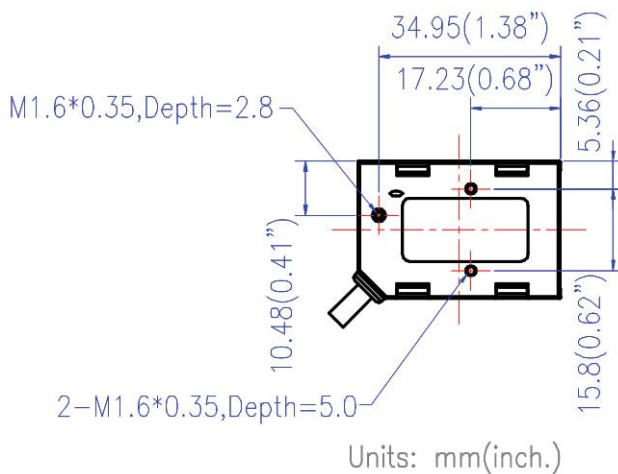
Figure 1: Screw Position
