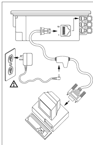
Figure 18: RS232 or Light Pen Interface
