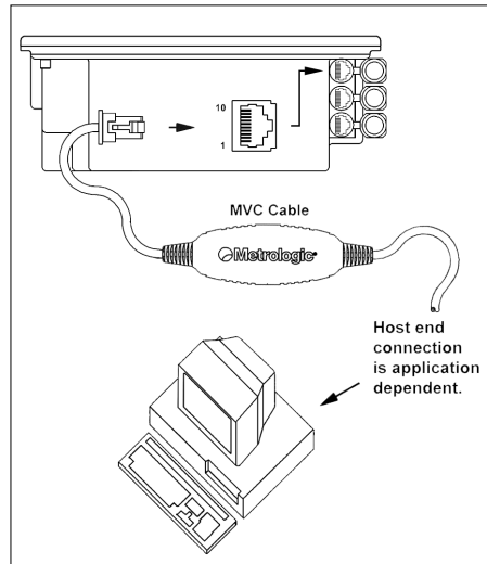
Figure 19: RS232/IBM, Interface
