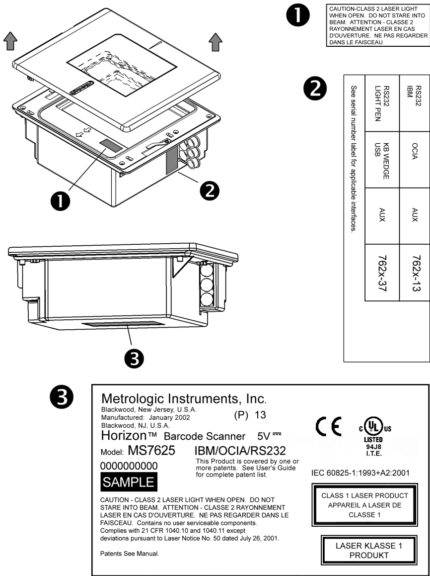
Figure 23: Label Locations
