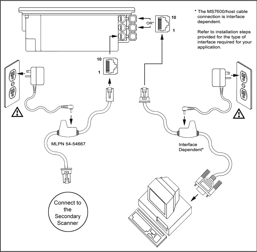
Figure 20: Connector Orientation (Top) Secondary Scanner Setup (Bottom)
