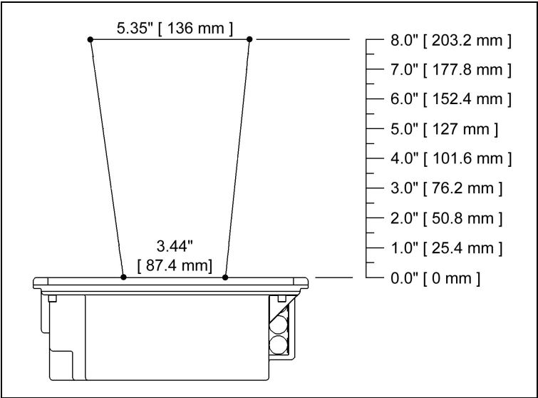
Figure 28: Scan Volume in Plane Perpendicular to Flow
