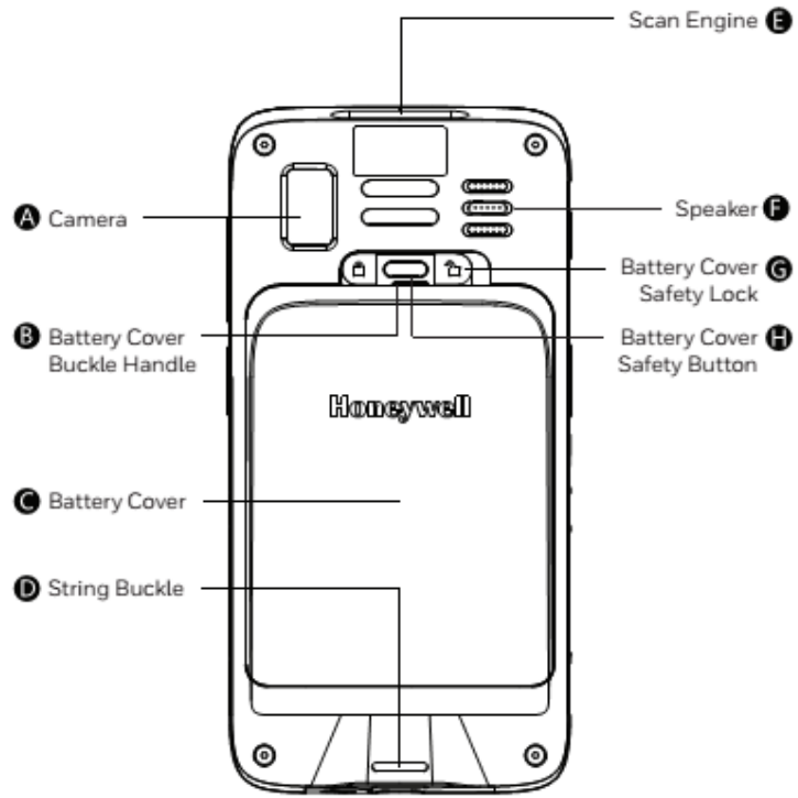
EDA51-X rear view
