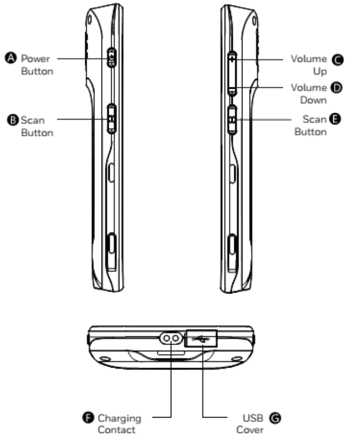
EDA51-X side and bottom views
